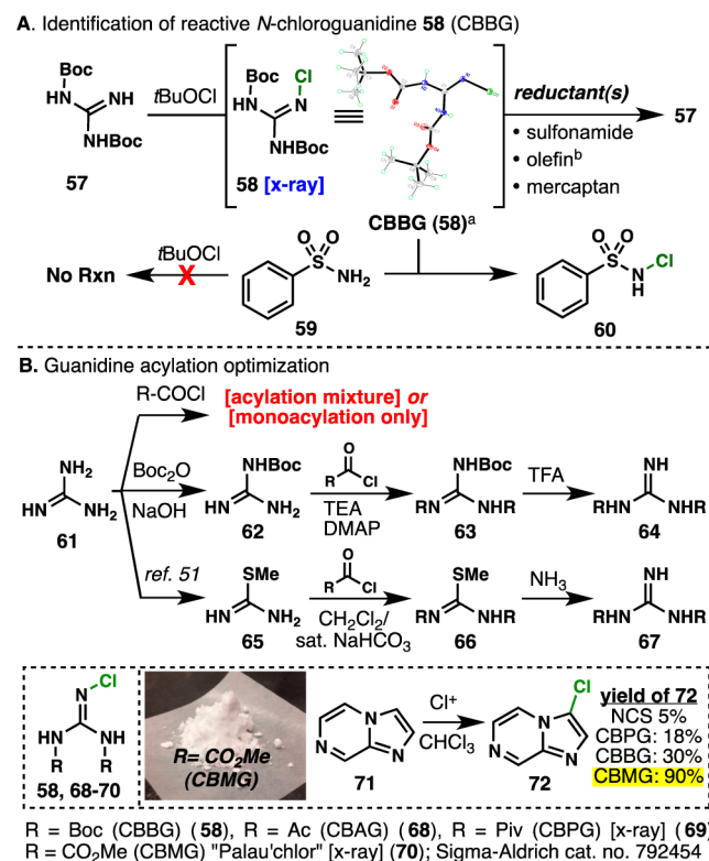
Scheme 6. Invention of Reactive yet Stable CBMG
