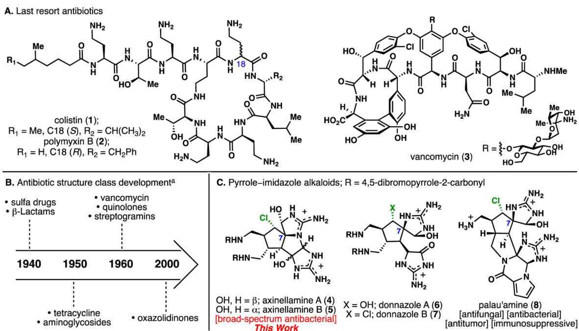
Figure 1. Antibiotic drug discovery. a Examples of drug class not necessarily introduced on the exact date depicted (modified from ref 11).
